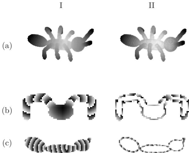
Figure 3. Top: 3D model of an ant. Column I: eccentricity transform of the ant. Column II: eccentricity transform of the border voxels of the ant. (a) Volume visualization of the eccentricity transform - darker means higher eccentricity, left and right use different gray value scales. (b) Cut along plane x = \text{const} . (c) Cut along plane z = \text{const} . (a) and (b) use the same gray value assignment as in Figure 1. approach for using ECC histograms to match 2D Shapes can be found in [11].
