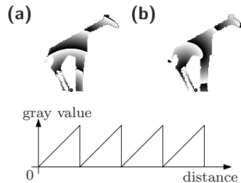
Figure 1. An example of (a) Euclidean and (b) geodesic distance function, for some starting point p_0 .
