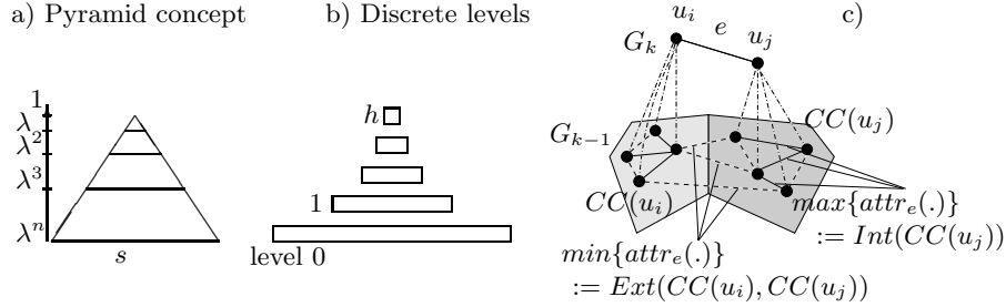
Fig. 1. (a,b) Multiresolution pyramid. (c) Internal and external contrast.
