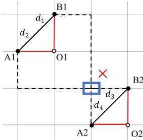
(c) Contradiction to planarity of the graph G.
